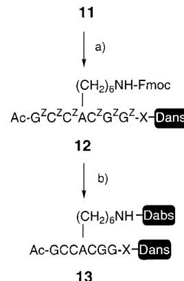
Scheme 3. Synthesis of doubly labeled PNA conjugate 13 . a) EDC, HOAt, Dans-X-H, DMF, \text{CH}_2\text{Cl}_2 ; b) 1. DMF/morpholine (1/1); 2. m -cresol/MeSMc/TFMSA/TFA (1/1/1/10), 66 % (based on 11 ); c) Dabs-Cl (4 equiv), sat. \text{NaHCO}_3 , DMF, 50 %. Dabs = 4-dimethylaminoazobenzene-4'-sulfonyl, Dans = 5-dimethylaminonaphthalene-1-sulfonyl, EDC = \text{Me}_3\text{N}(\text{CH}_2)_3\text{N}=\text{C}=\text{NEt} \cdot \text{HCl} , HOAt = 1-hydroxy-7-azabenzotriazole, TFMSA = trifluoromethanesulfonic acid, X = \text{NHCH}_2\text{CH}_2\text{NH} .
